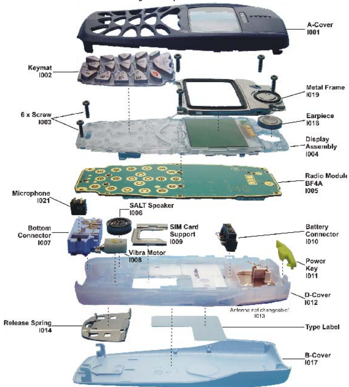
Figure 1: Exploded view of RH-9
